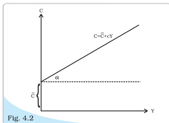
Consumption function with intercept \bar{C} .
