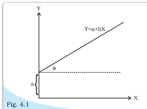
Intercept form of the linear equation.
