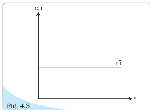
Investment function with I as autonomous.
