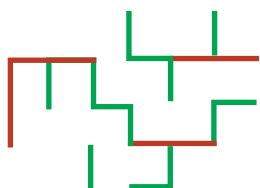
Fig. 5.21: A maze
